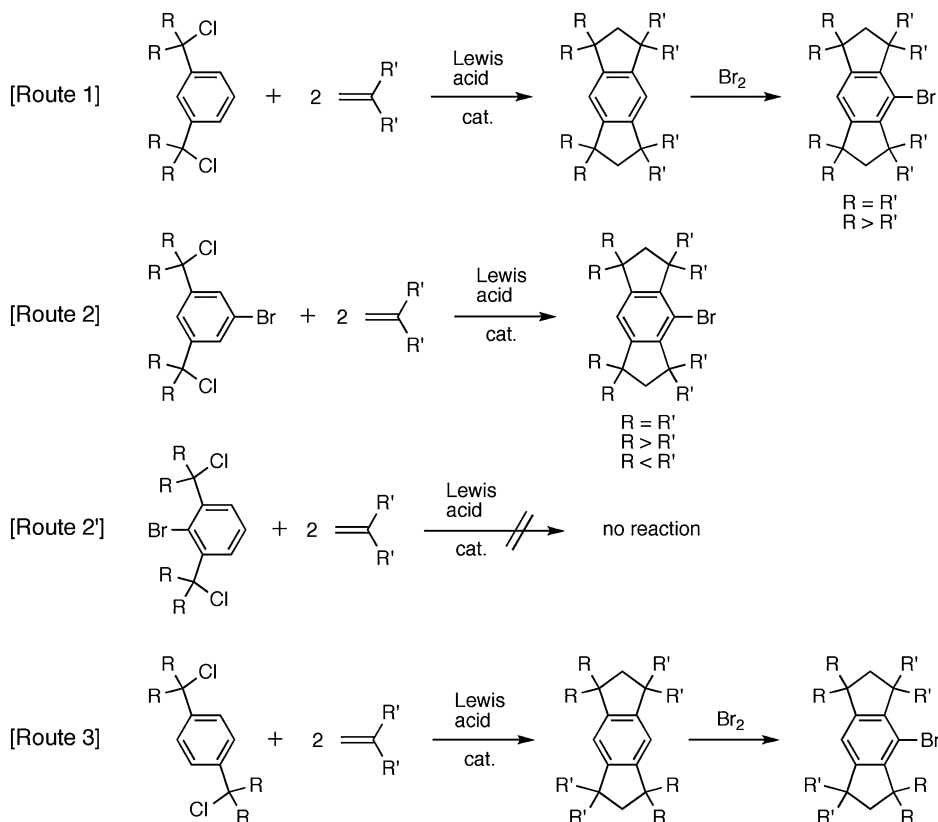
Scheme 1. Synthetic routes to Rind-Br.
