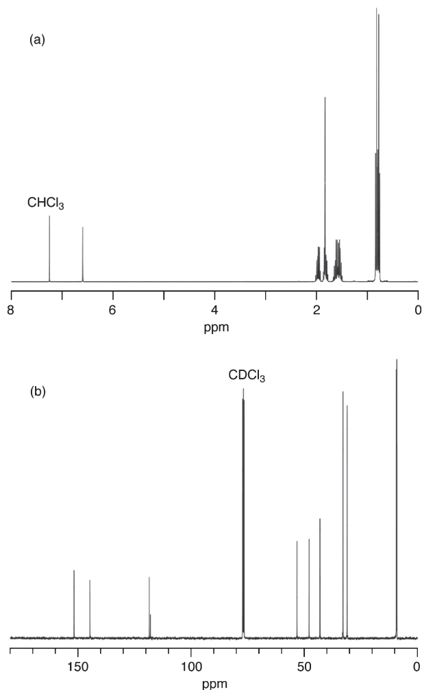
Figure 4. (a) ^1\text{H} and (b) ^{13}\text{C} NMR spectra of Eind-Br ( \text{CDCl}_3 , 298 K).
