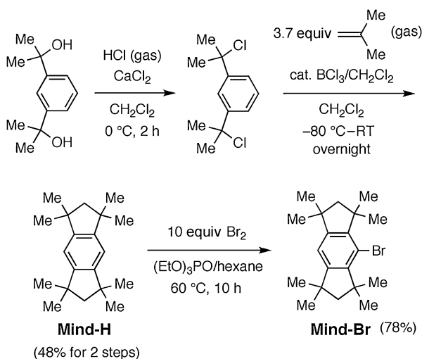
Scheme 3. Synthesis of Mind-Br.
