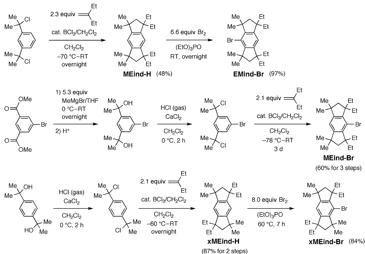
Scheme 4. Synthesis of EMind-Br, MEind-Br, and xMEind-Br.
