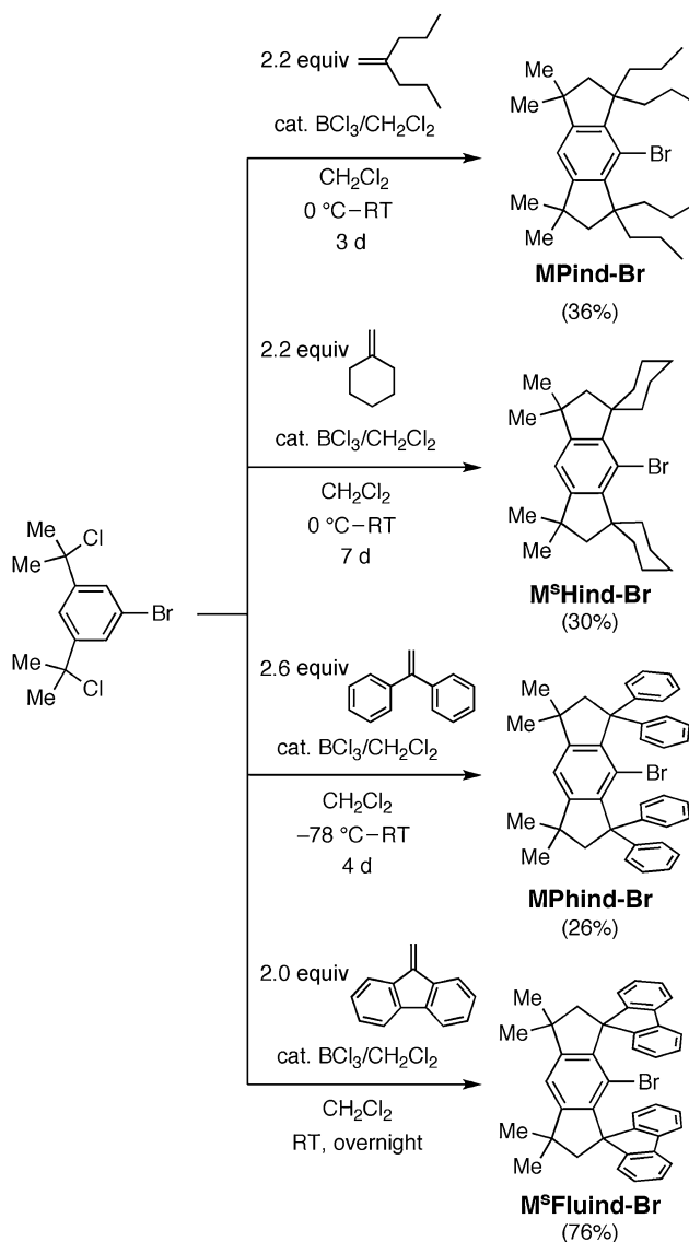
Scheme 6. Synthesis of MRind-Br.
