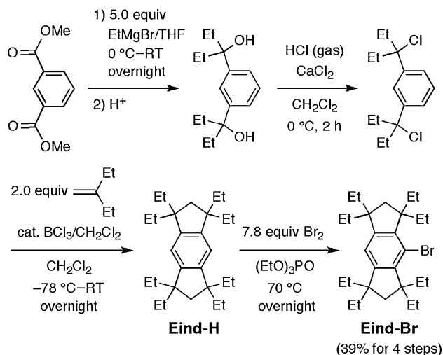
Scheme 2. Synthesis of Eind-Br.
