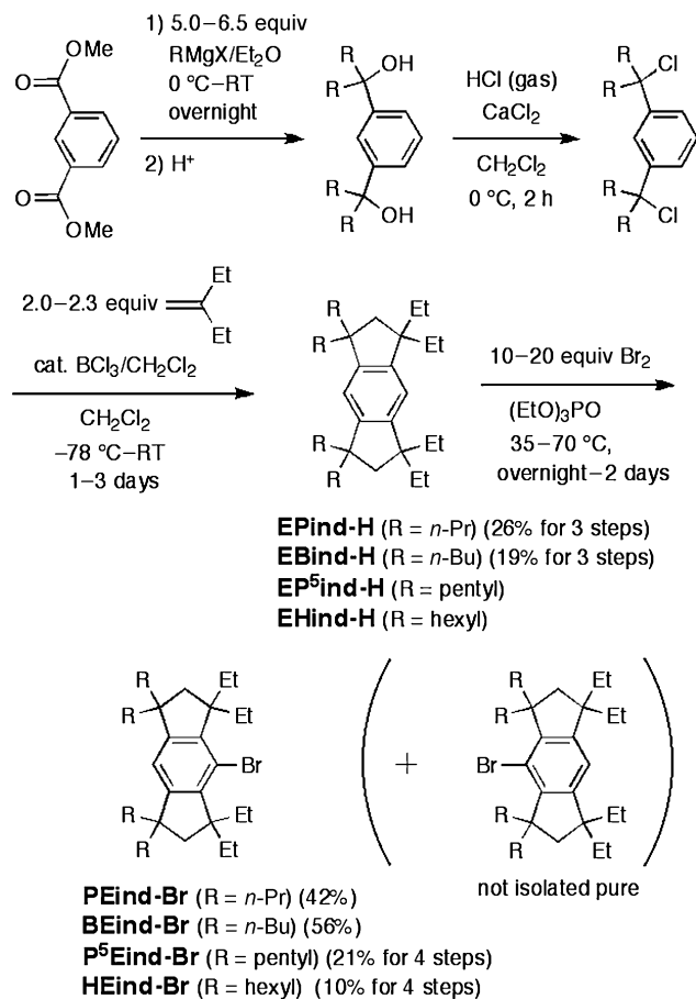
Scheme 5. Synthesis of REind-Br.
