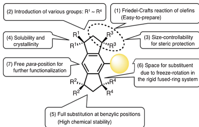
Figure 2. Features of Rind groups.
