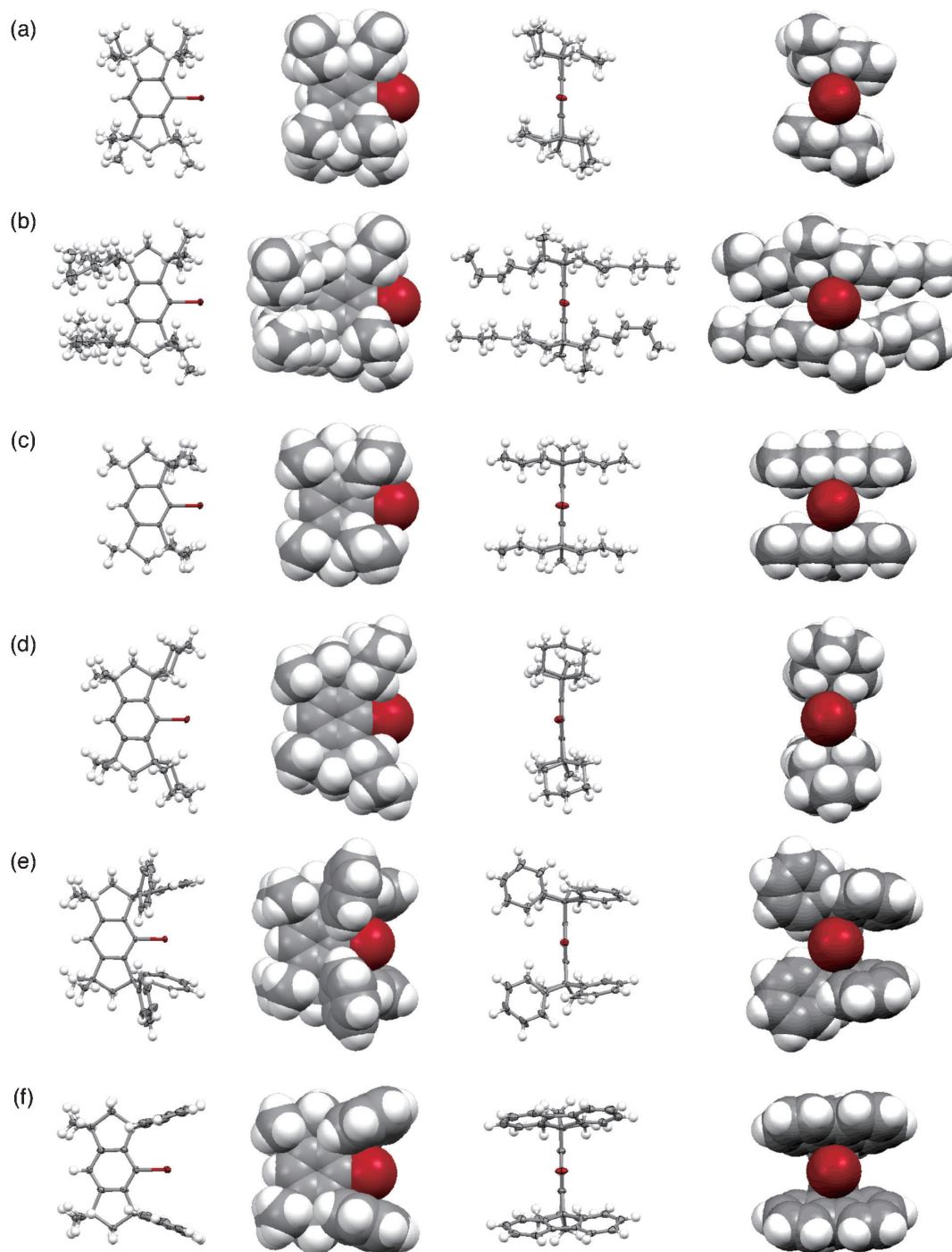
Figure 3. Molecular structures of (a) Eind-Br, (b) HEind-Br, (c) MPind-Br, (d) M s Hind-Br, (e) MPhind-Br, and (f) M s Fluind-Br: top views (left), front views (center), and space filling models (right).
