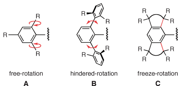
Figure 1. Three types of bulky aryl groups: 2,4,6-trialkyl-phenyl groups (A), 2,6-bis(2,6-dialkylphenyl)phenyl groups (B), and octa-R-substituted fused-ring aryl groups (C).
